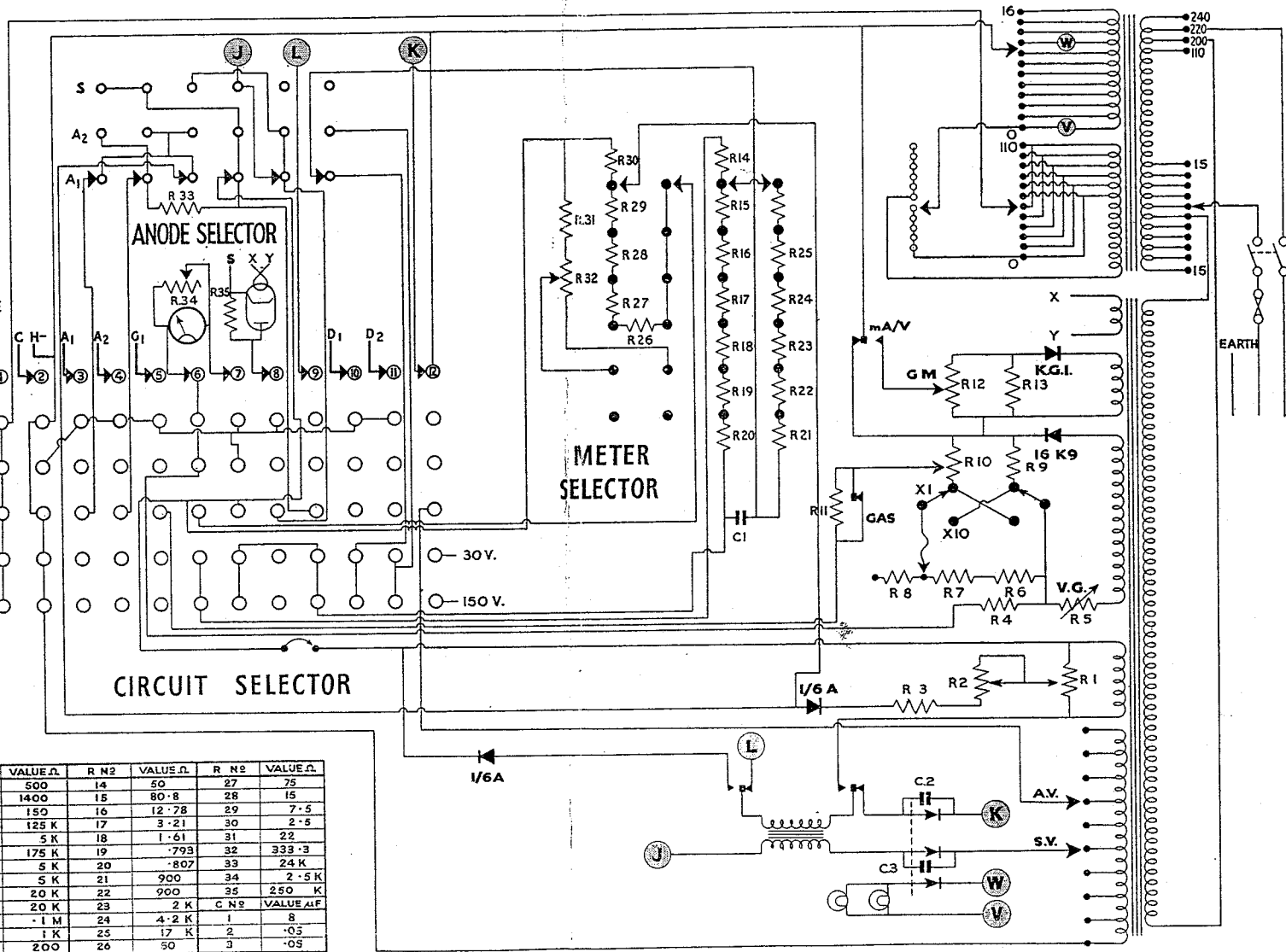
ELECTRODE LEAKAGE
