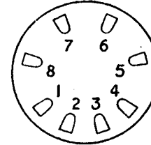
P-TYPE BASE (85C)
