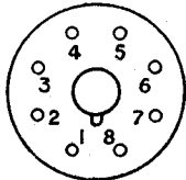
INTERNATIONAL OCTAL (A08)
