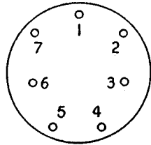
BRITISH SEVEN PIN (B7)
